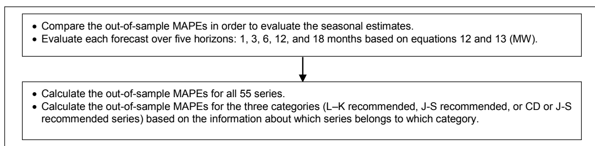
Fig. C.4. Accuracy Assessment
