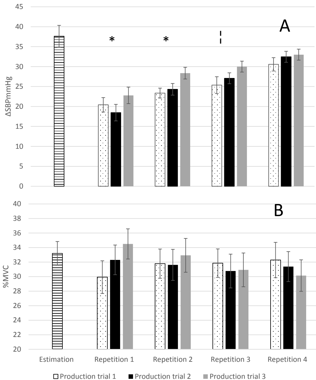
Fig. 2 One way ANOVA between \Delta SBP (mean \pm SEM) and %MVC (mean \pm SEM) during the estimation task and production trials 1-3. Panel A * = significant differences between production trials 1-3 and estimation task ( p < 0.05 ). † = significant differences between estimation task and production trials 1-2 ( p < 0.05 ). Panel B No significant differences between %MVC estimation task and %MVC production trials 1-3, reps 1-4.
